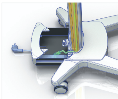
Lockable electrical box – ensures secure storage of multiple sockets and power supply units and protects against unauthorized access
