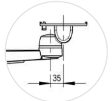
universal adapter – up to 14 kg / 30.6 lbs
