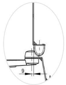
VESA 75 / 100, universal – up to 14 kg / 30.6 lbs
