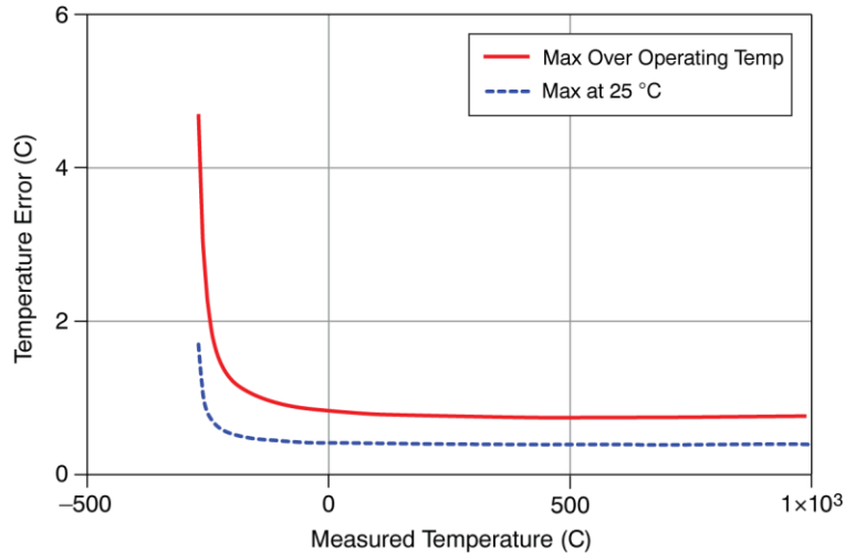
Temperature error of E type thermocouple
