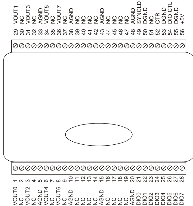
Figure 5. USB-3103 signal pin out
