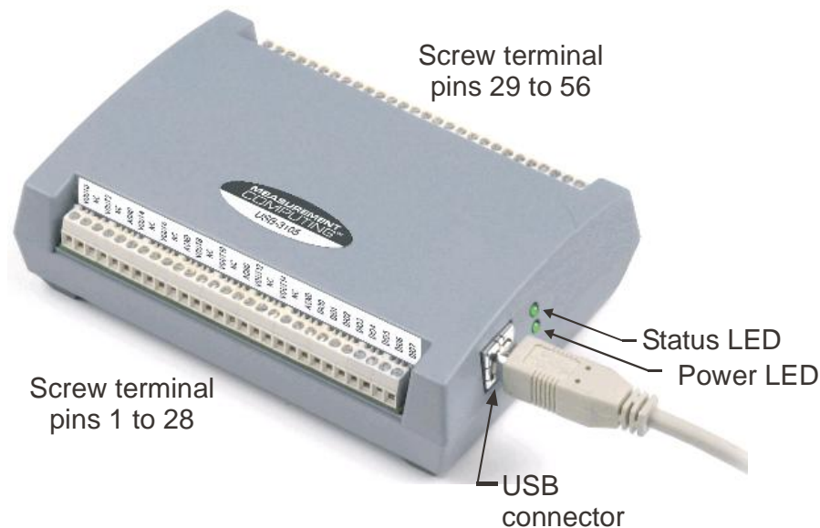
Figure 3. USB-3105 external components
