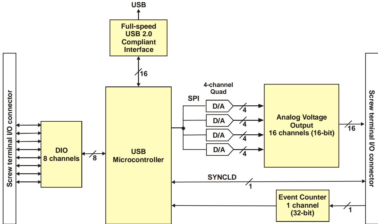
Figure 2. USB-3105 block diagram
