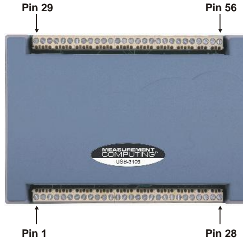
Figure 4. USB-3105 screw terminal pin numbering
